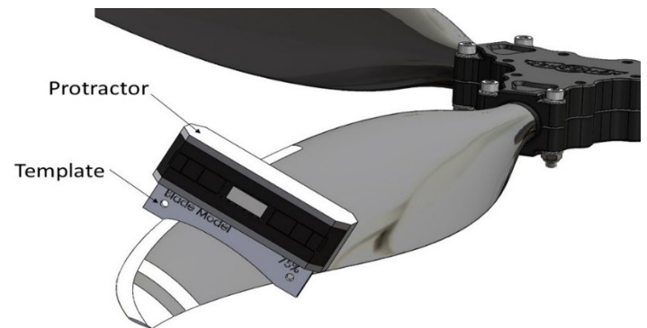
FIGURE 3. PITCH SETTING WITH PROTRACTOR
